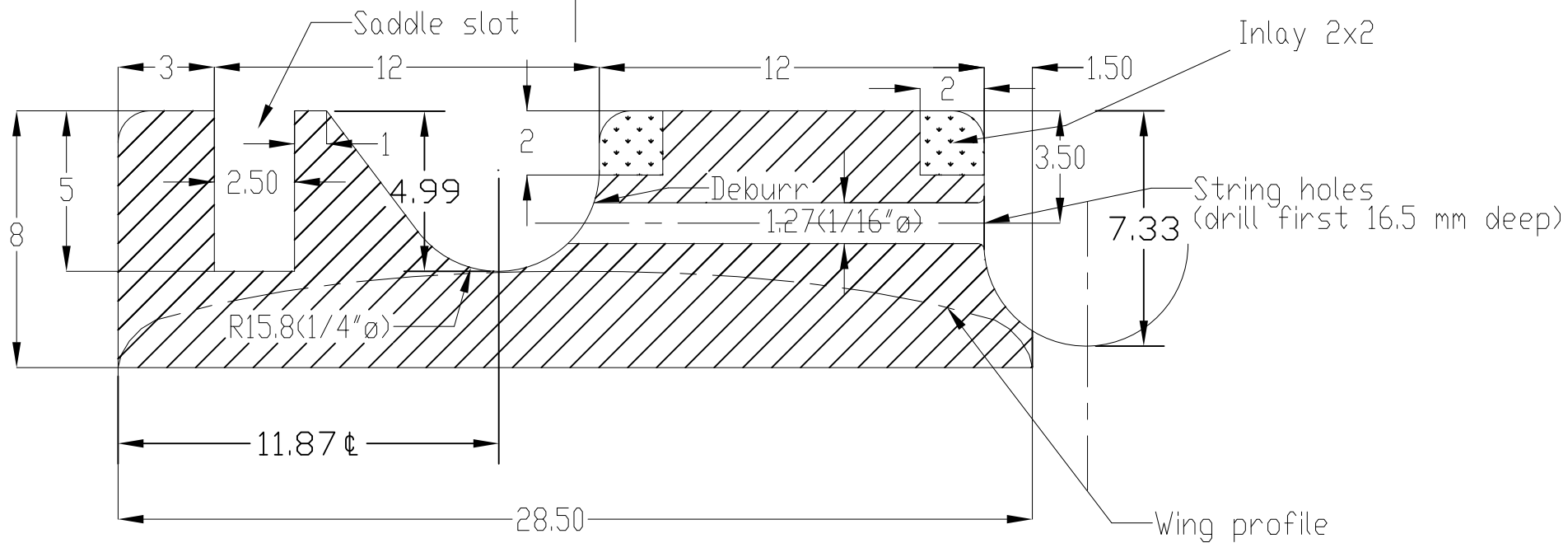
Bridge
